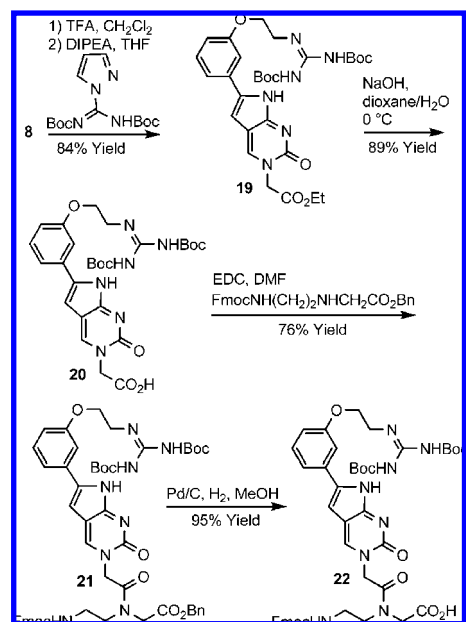
Scheme 3. Synthesis of mmguaPhpC Monomer
