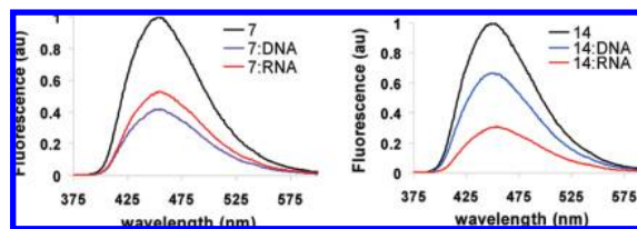
Figure 3. Fluorescence emission spectra of sequences 7 and 14 containing mmguaPhpC when hybridized to DNA and RNA.
