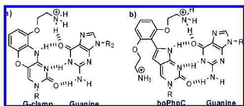
Figure 1. Previously studied cytosine analogues, based on the phenoxazine and PhpC nucleobases, capable of forming a fourth hydrogen bond to guanine: (a) phenoxazine-based G-clamp and (b) phenylpyrrolocytosine-based boPhpC.
