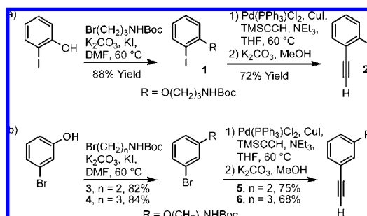
Scheme 1. Synthesis of Alkynes 2 , 5 , and 6
