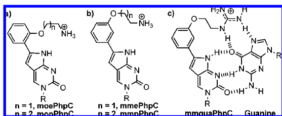
Figure 2. Structures of modified PhpCs designed to engage guanine with an additional hydrogen bond. (a) Previously studied moePhpC and newly synthesized mopPhpC; (b) meta-substituted PhpCs mmePhpC ( n = 1 ) and mmpPhpC ( n = 2 ); (c) proposed interaction of guanidino-PhpC (mmguaPhpC) with guanine.
