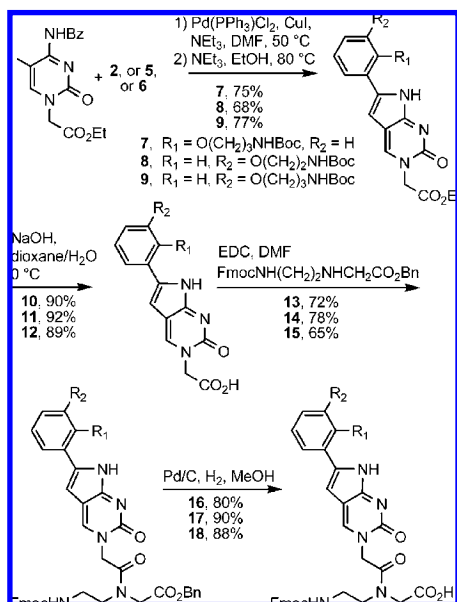
Scheme 2. Synthesis of Substituted PhPCs 16–18
